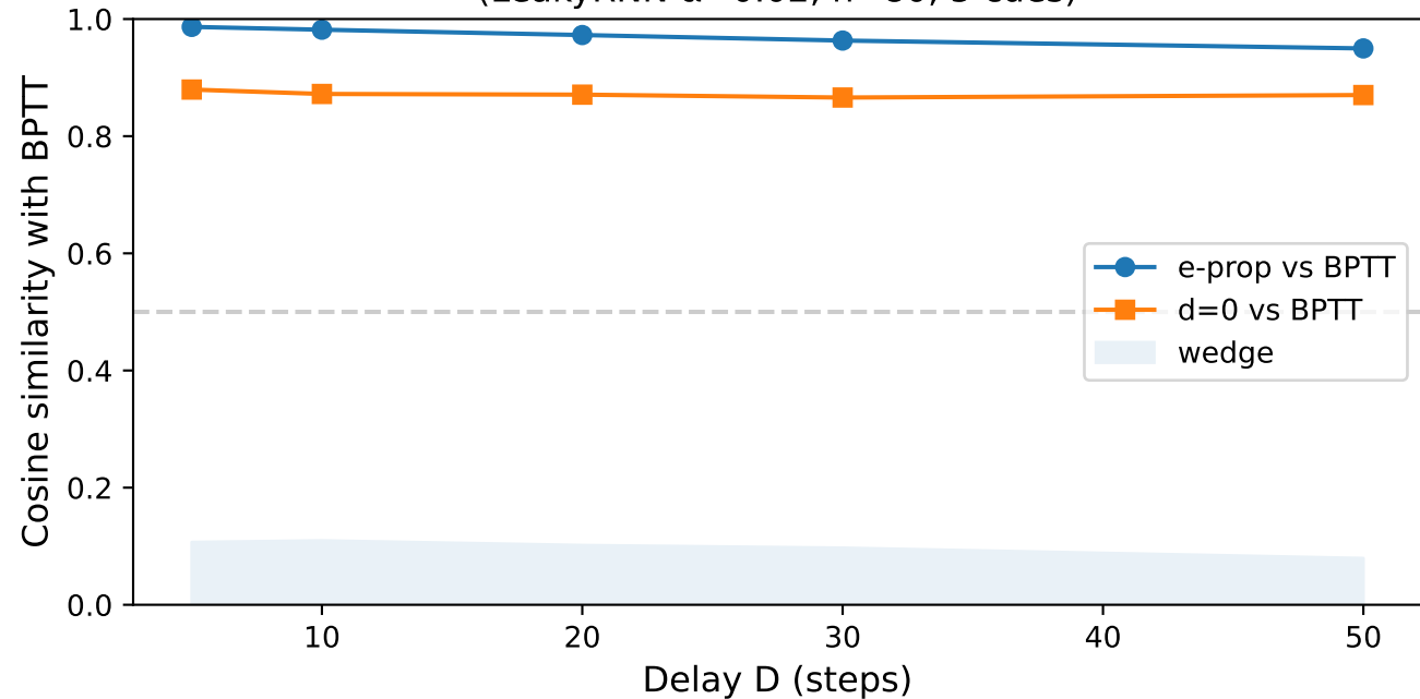
Cue Accumulation: Gradient Alignment vs Delay (LeakyRNN \alpha=0.02 , n=80 , 5 cues)
