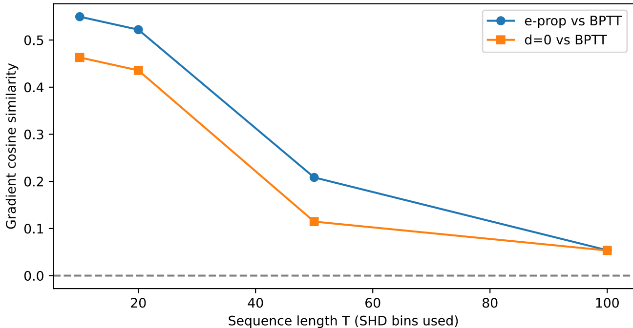
Gradient alignment — untrained deep ALIF ( 2 \times 256 ) \rho=0.98
