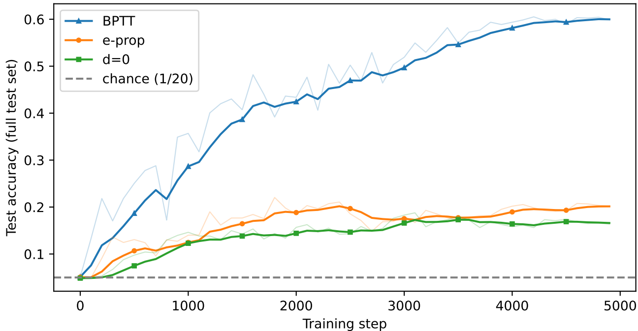
SHD — deep ALIF ( 2 \times 256 ) \alpha=0.9 \rho=0.98 \beta=0.02
