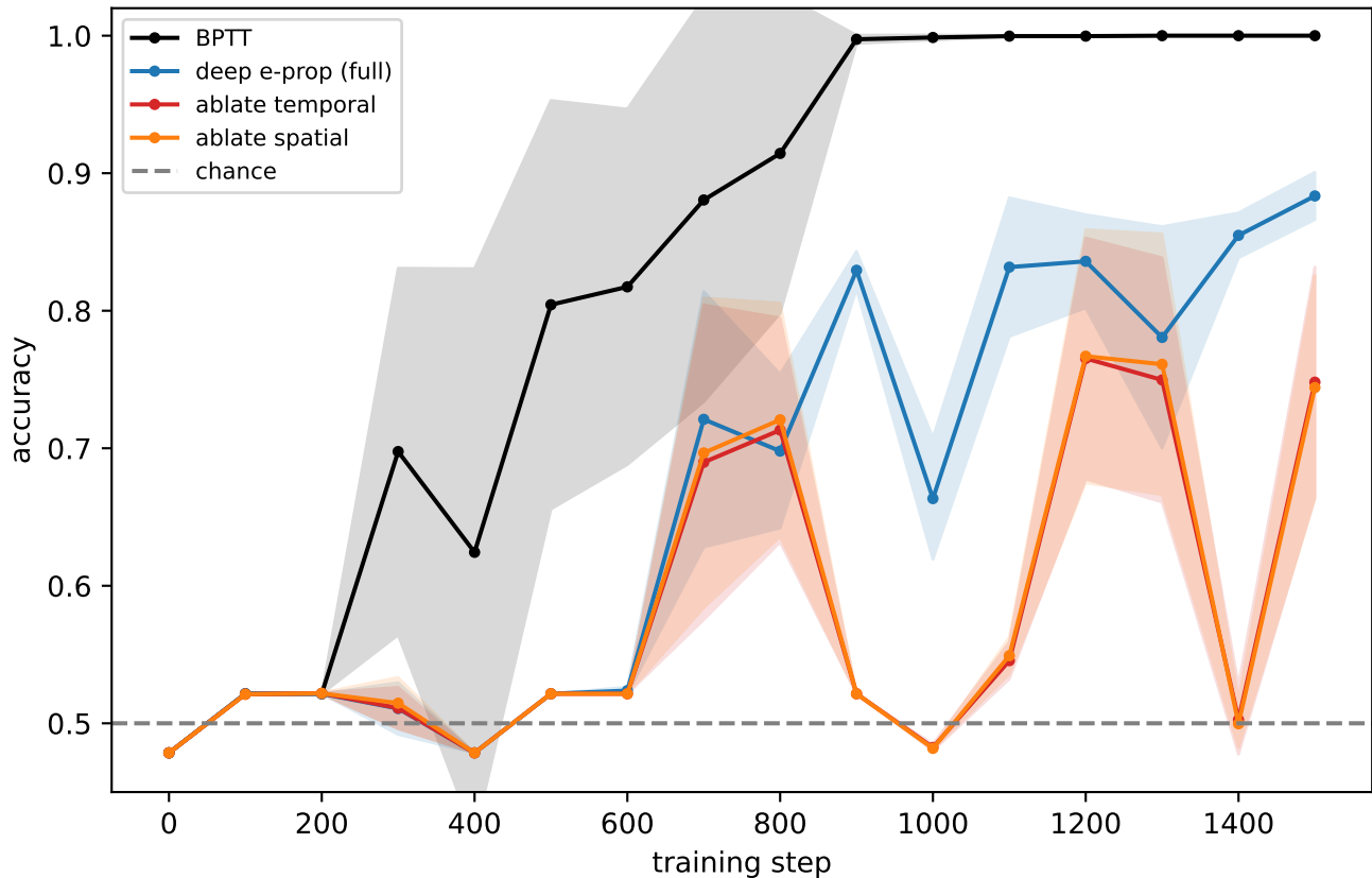
Learning the hierarchical task ( D=12 , \alpha=[0.5, 0.05] )
