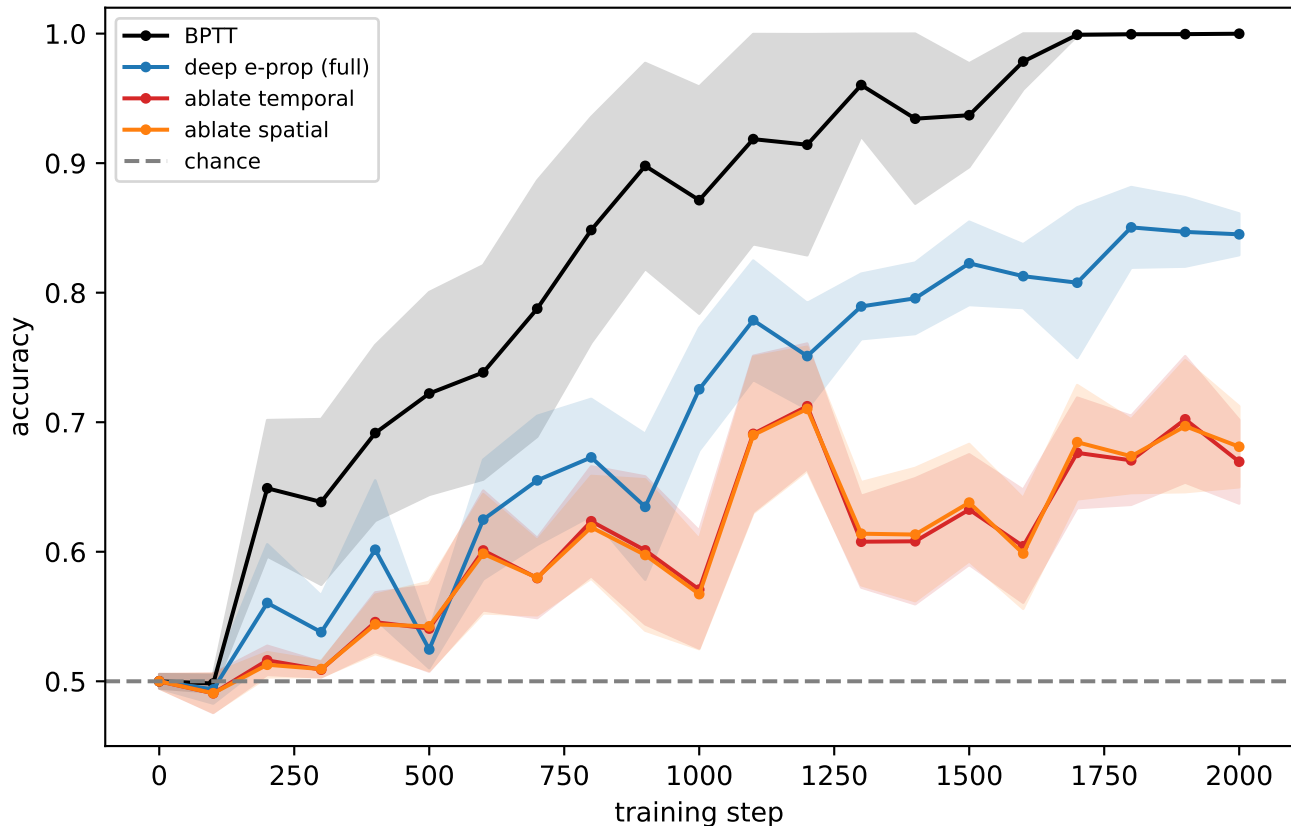
Learning the hierarchical task ( D=12 , \alpha=[0.5, 0.05] , n=6 seeds, \pm SEM)
