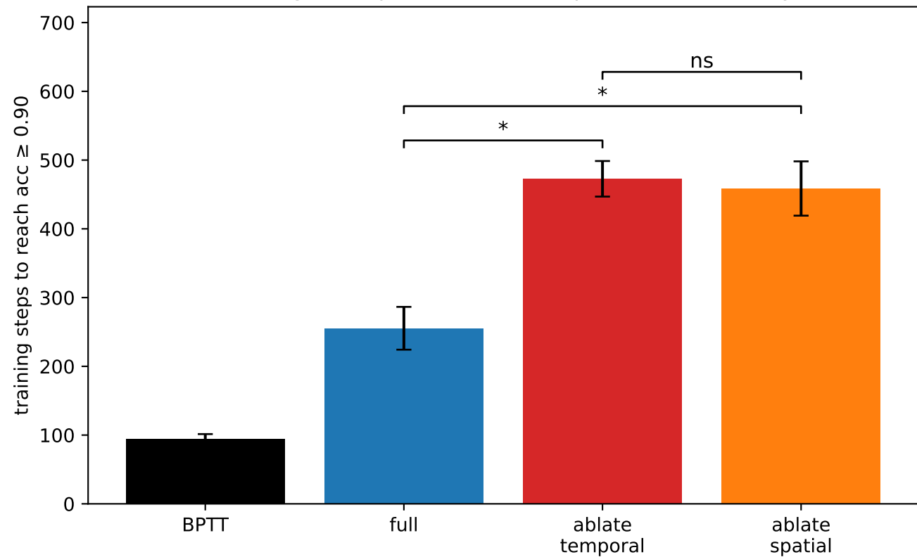
Convergence speed (Adam): steps to 90% accuracy
