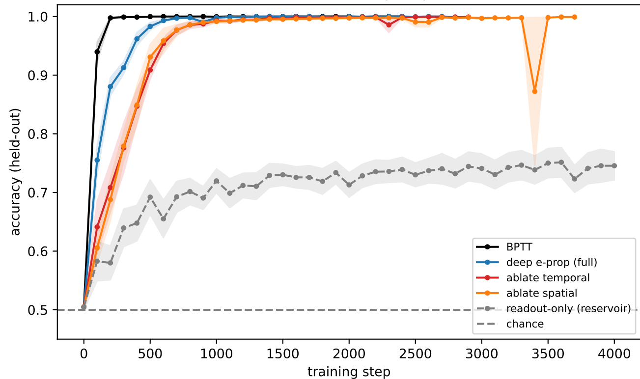
Adam (lr=1e-03): trainable rules converge equal; reservoir floors below
