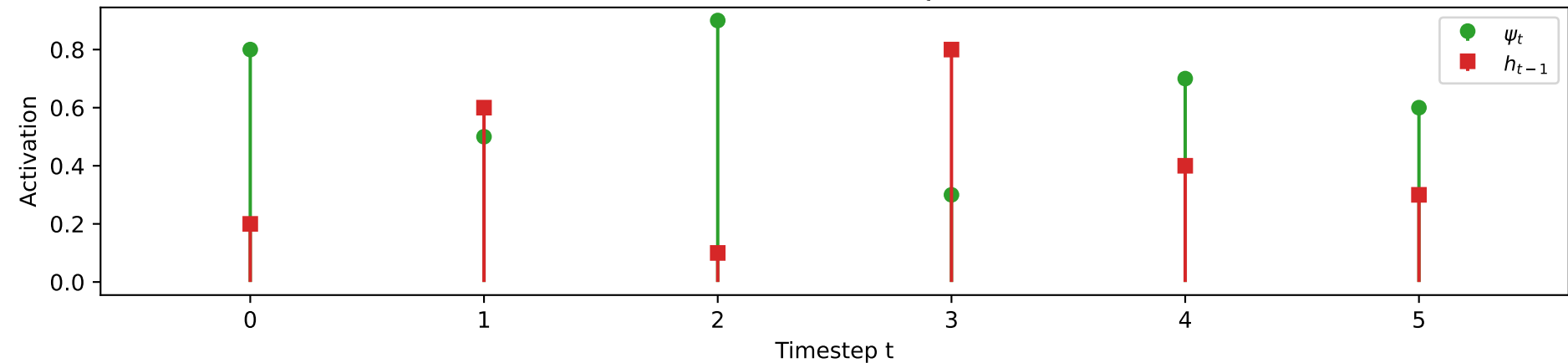
Inputs to trace: \psi_t = 1 - h_t^2 and h_{t-1}
