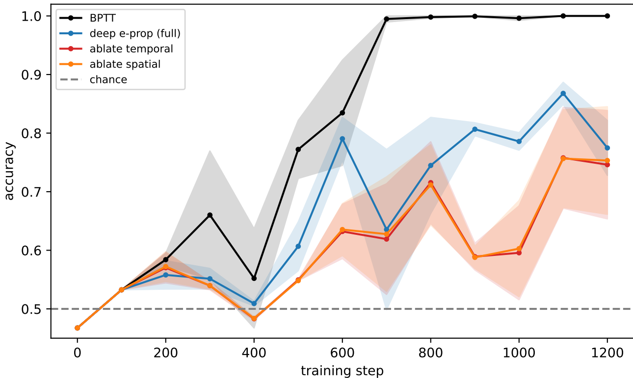
Exp 5.2 — BPTT \geq full e-prop > controls (D=10)
