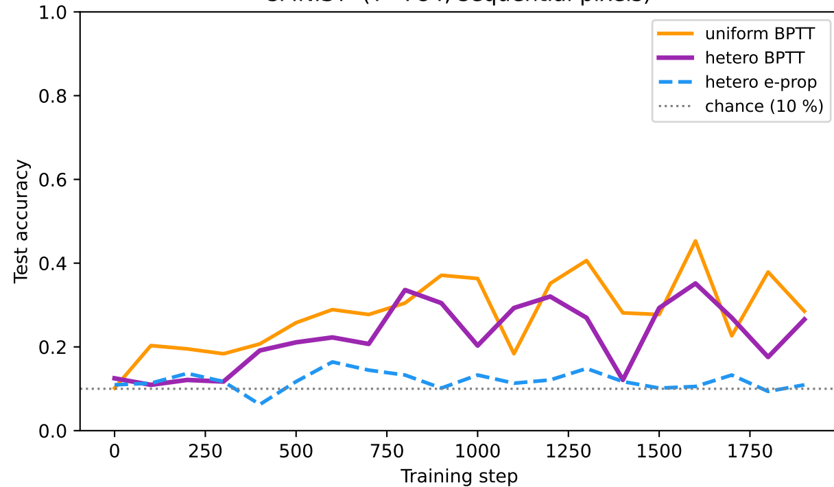
sMNIST ( T=784 , sequential pixels)
