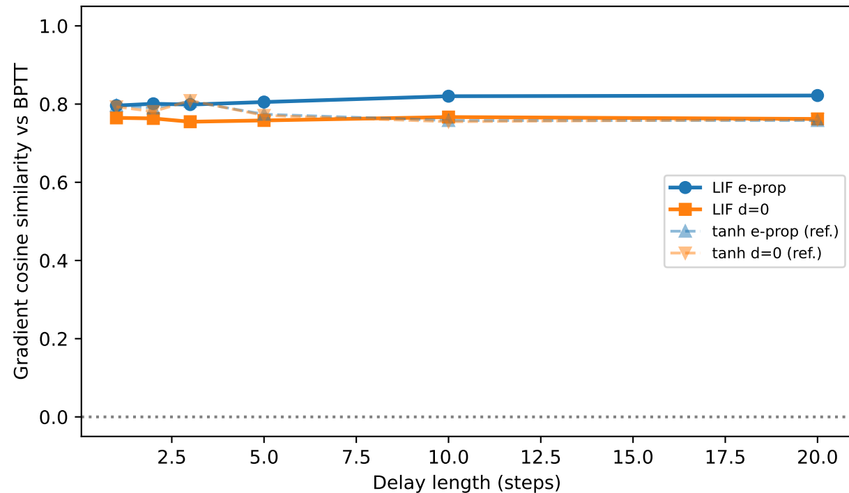
LIF vs tanh: e-prop/d=0 gradient alignment
