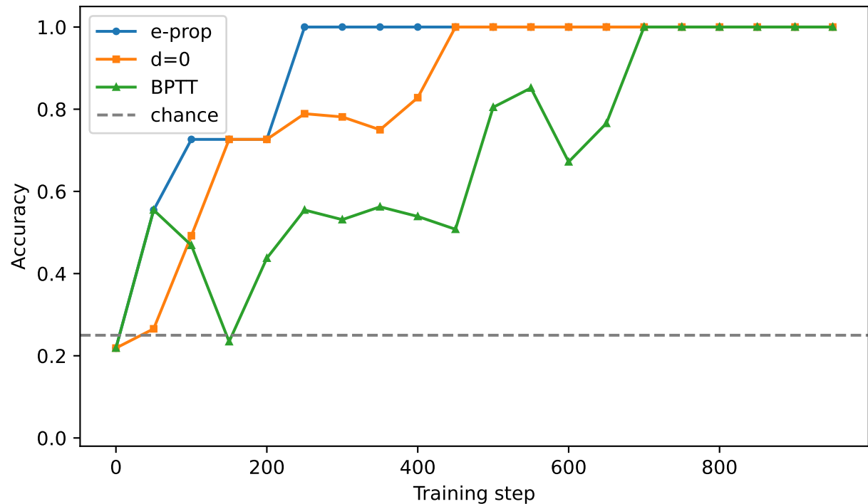
LIF store-and-recall (delay=5, n=100)
