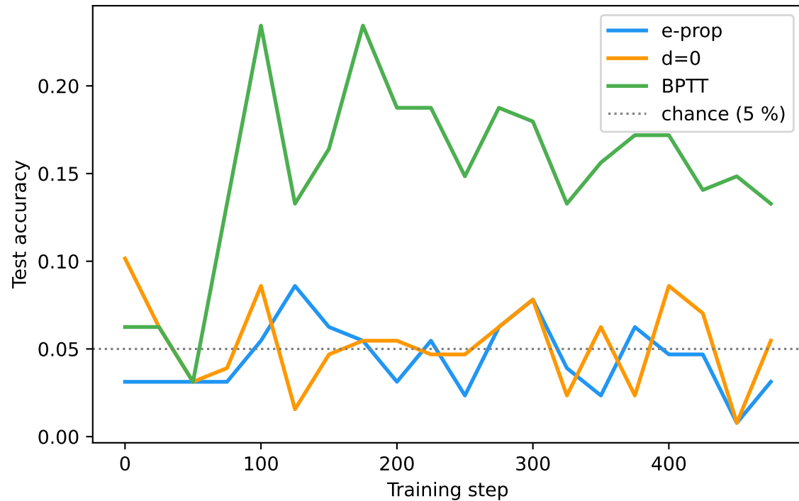
SHD learning curves (LIF, n_rec=128)
