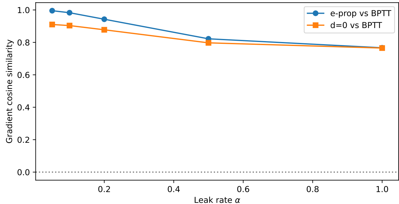
Leaky RNN: e-prop vs d=0 gradient alignment (delay=5)
