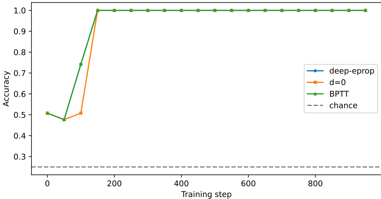
Deep e-prop learning curves (2-layer, delay=2)
