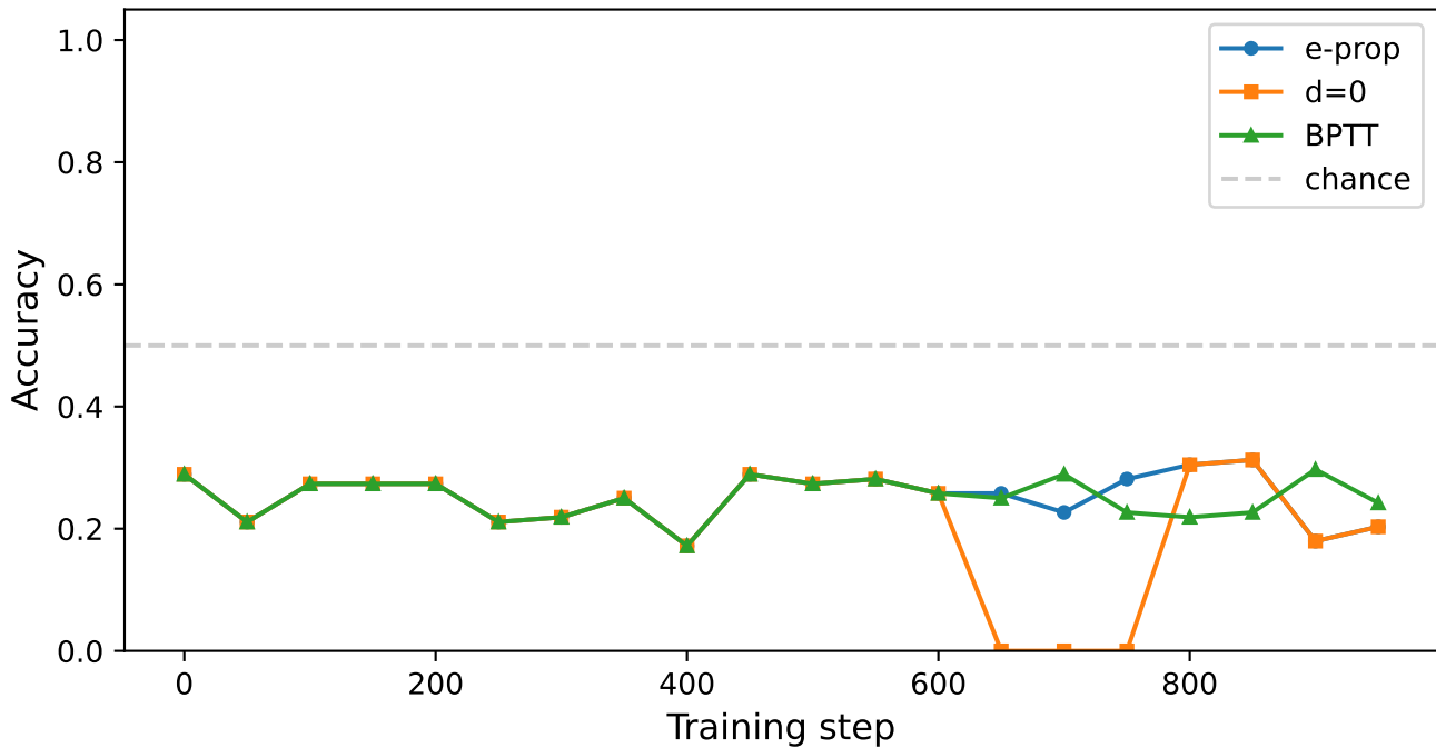
Leaky RNN Learning Curves ( \alpha=0.1 , D=5 )
