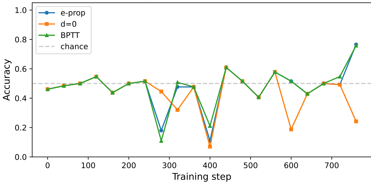
Cue Accumulation — Qualitative Illustration (LeakyRNN \alpha=0.02 , D=50 , 5 cues)
