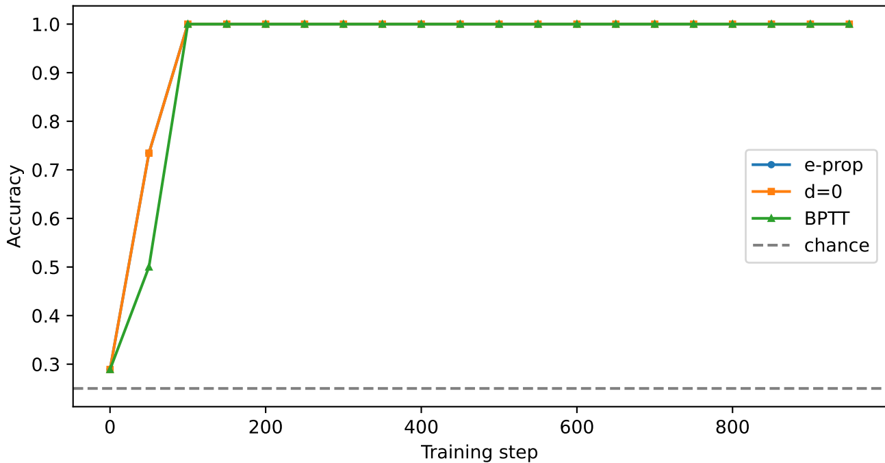
Store-and-recall learning curves (single layer, delay=2)
