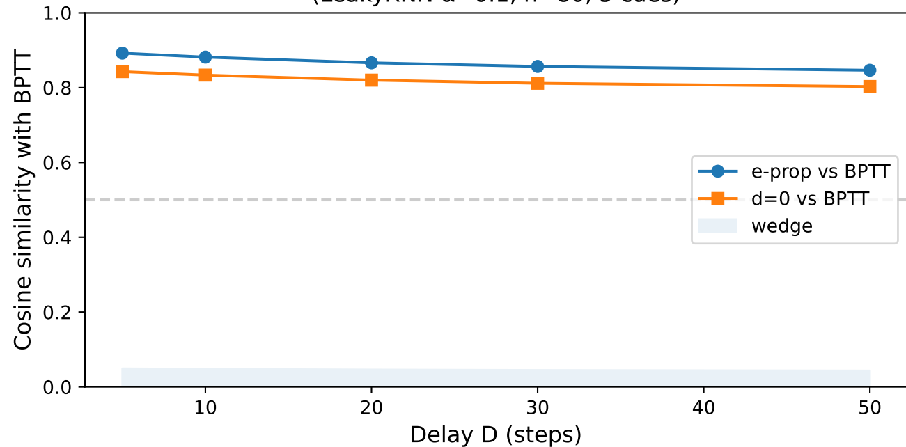
Cue Accumulation: Gradient Alignment vs Delay (LeakyRNN \alpha=0.1 , n=80 , 5 cues)
