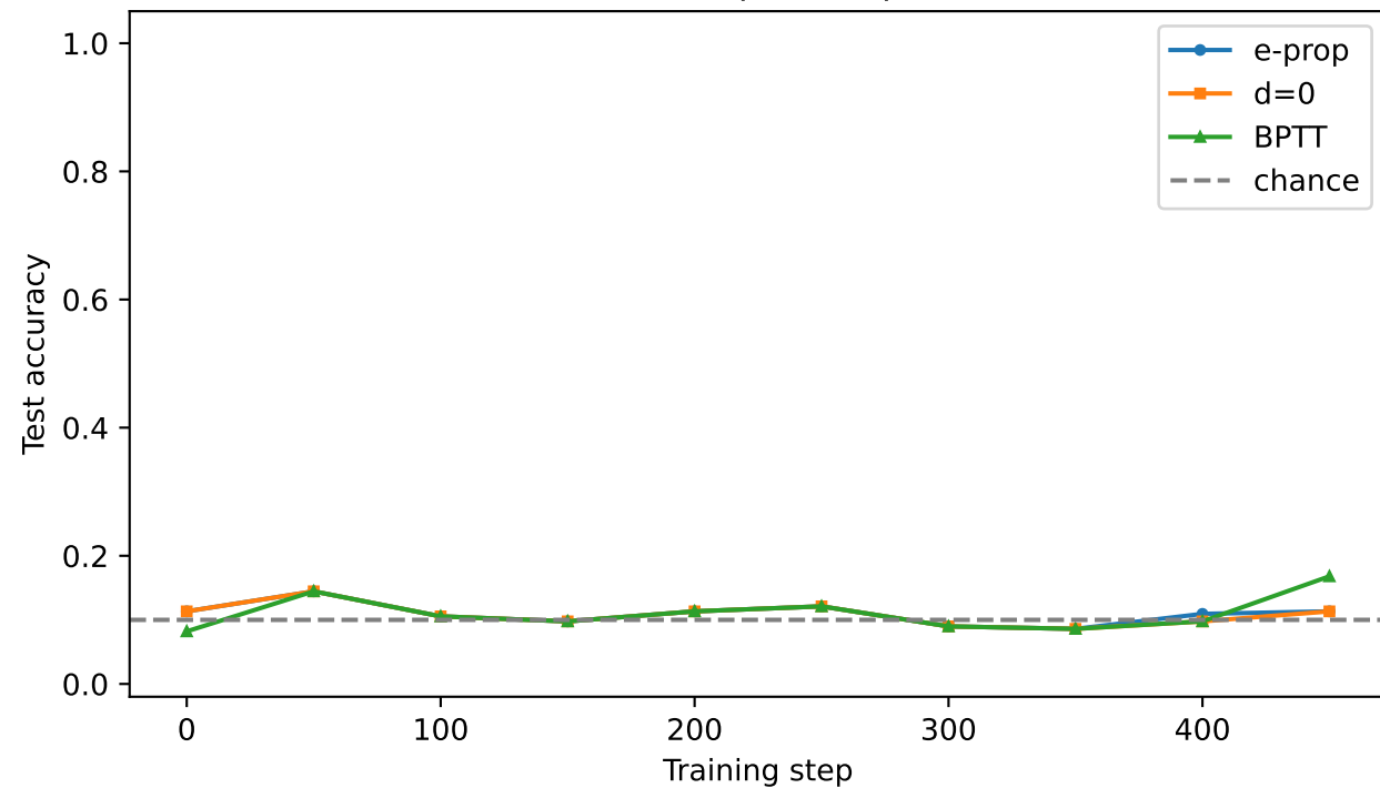
smNIST (sequential pixels)
