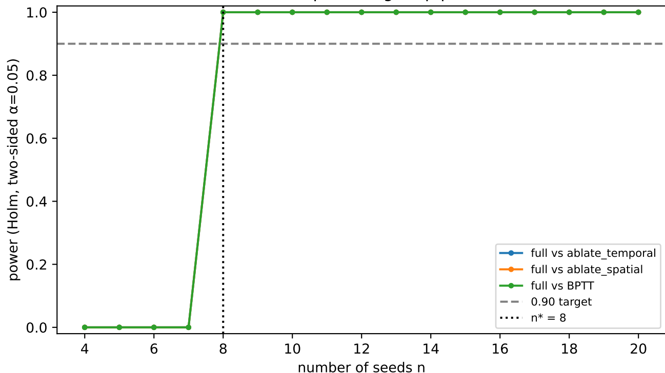
Simulation power vs #seeds (headline test = paired sign-flip permutation)
