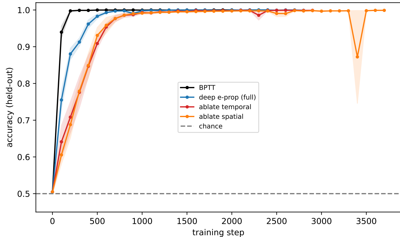
Adam (lr=1e-03): equal final accuracy, credit quality sets speed
