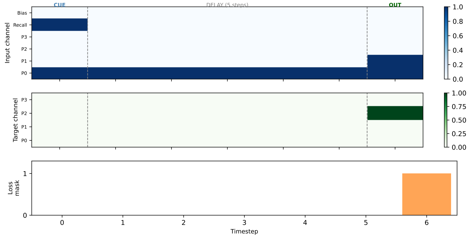
Fig 1 — Store-and-recall task (cue / delay / output)
