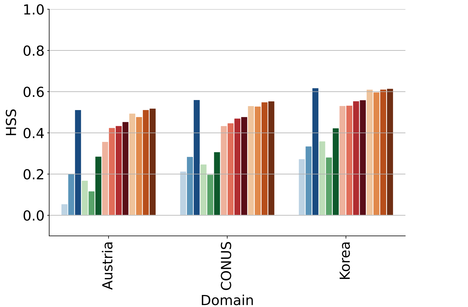
(a) Precipitation Detection ( 0.1 \text{ mm h}^{-1} < P )
