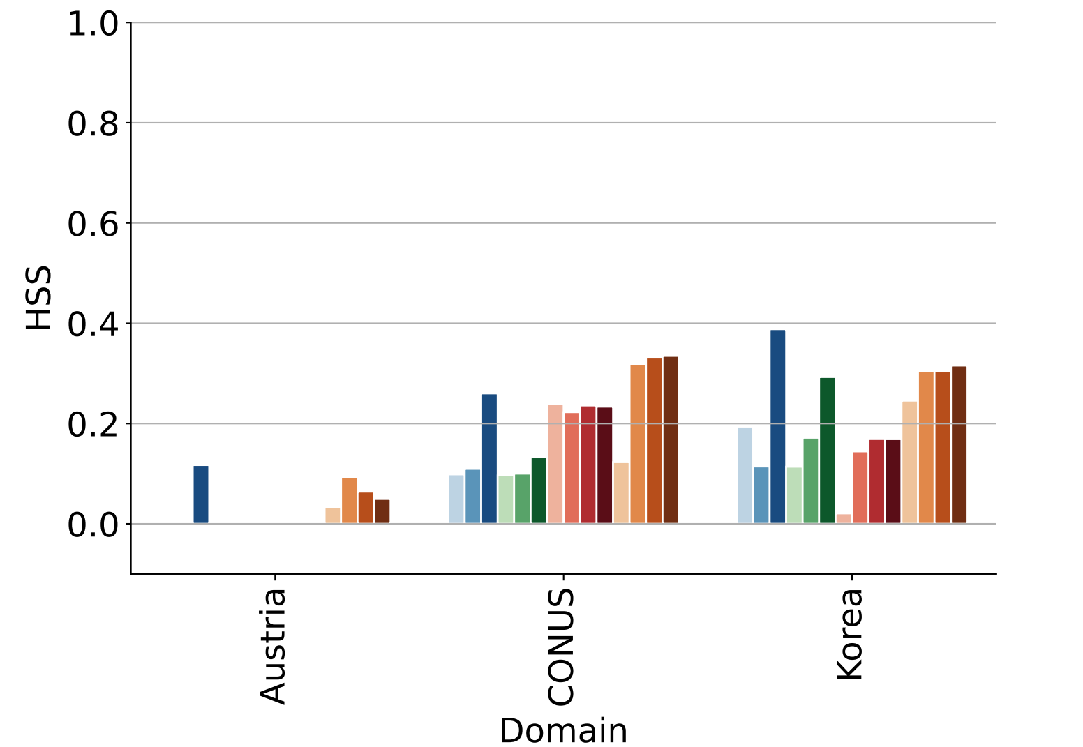
(b) Heavy Precipitation Detection ( 10 \text{ mm h}^{-1} < P )
