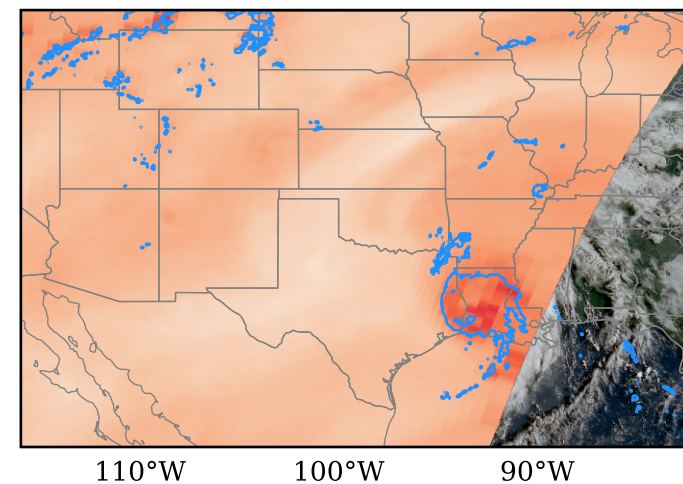
(f) 183.3 +/- 3.0 GHz, QH Pol.
