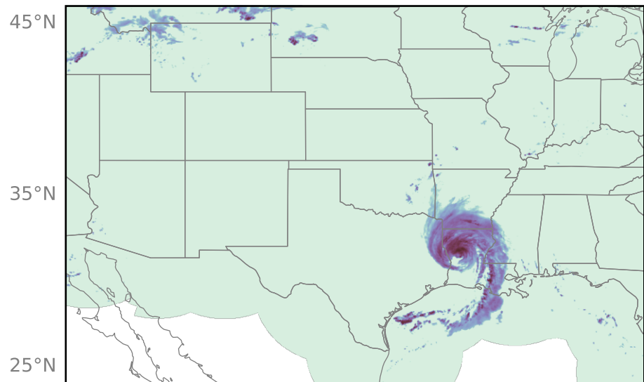
(a) Surface precipitation
