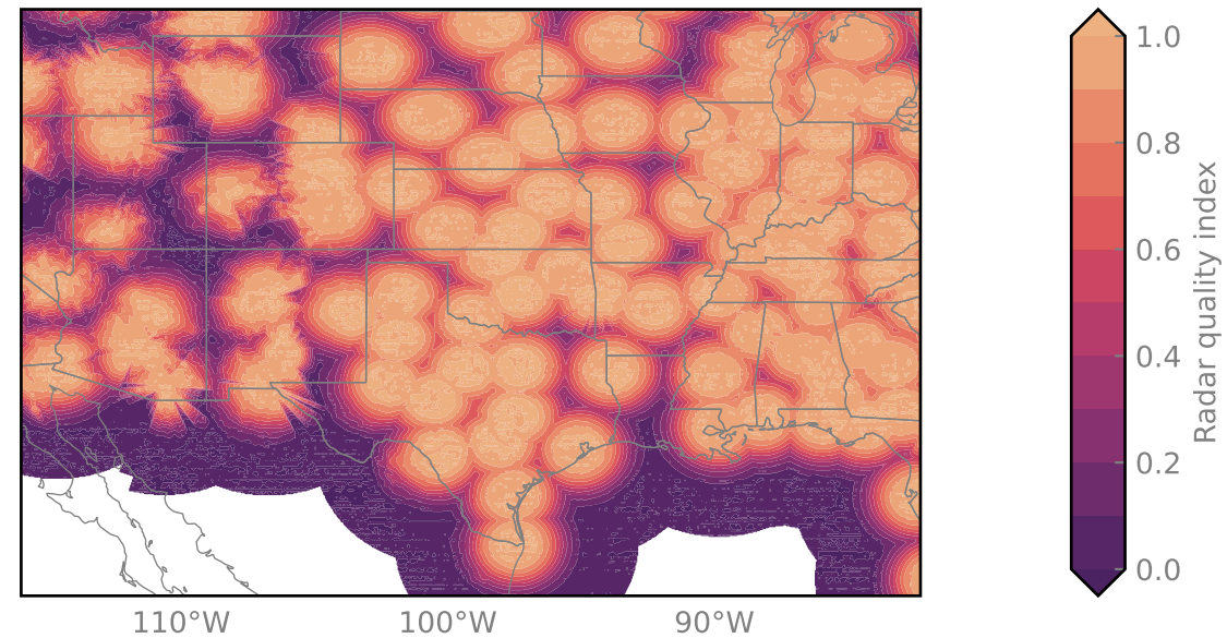
(b) Radar quality index
