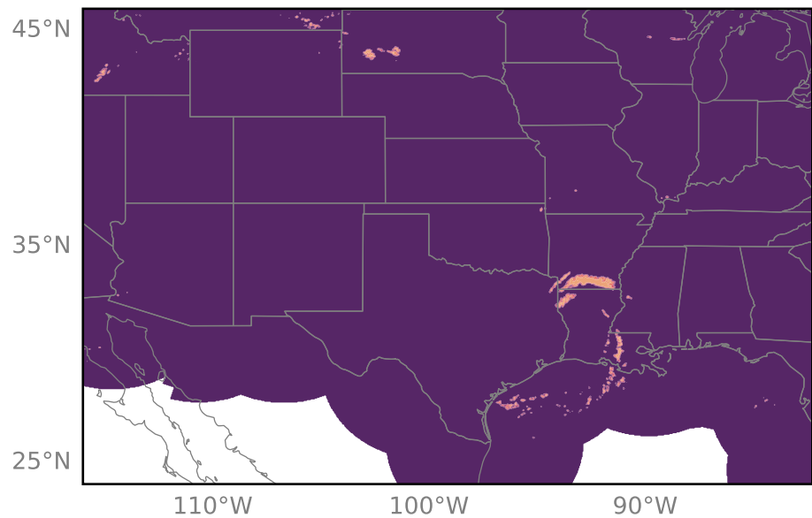
(c) Convective fraction
