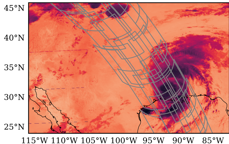
(c) Gridded IR obs.
