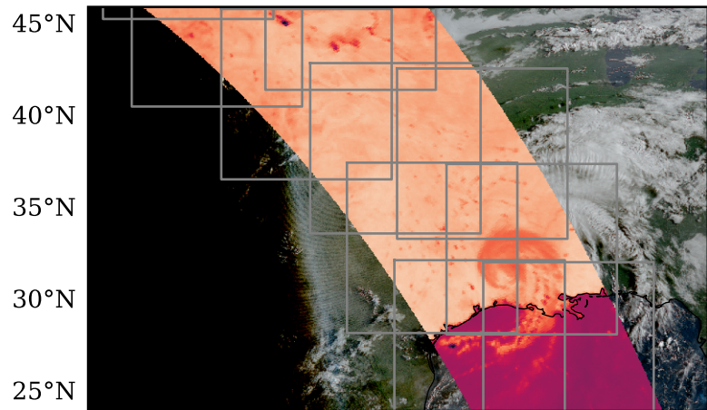
(c) Gridded IR obs.
