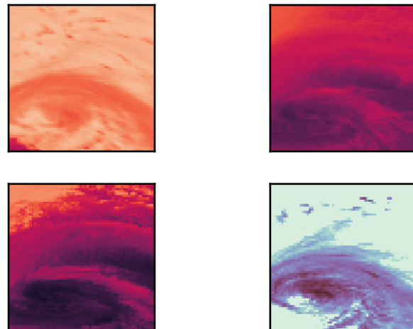
(f) On-swath training samples
