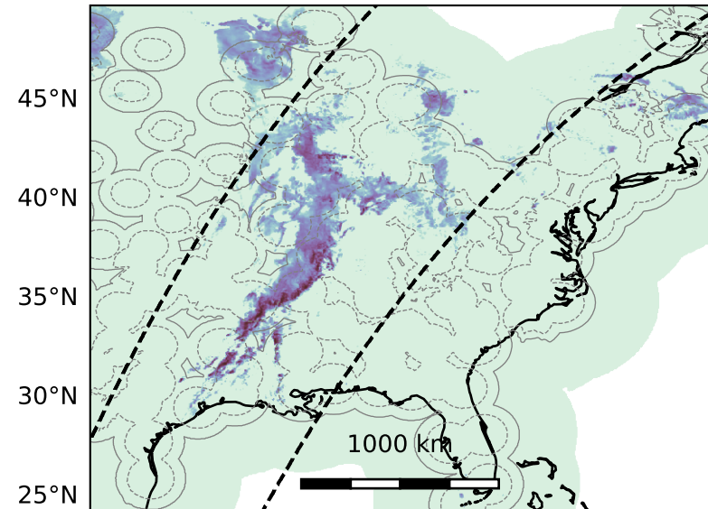
(a) Reference
