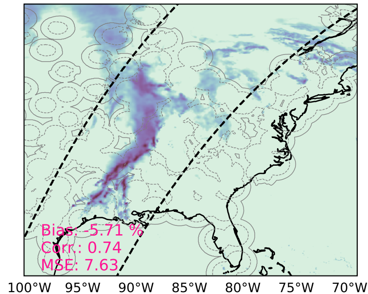
(e) SatRain (Geo)
