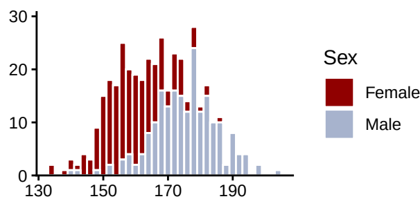
Figure 1: Distribution of height (in cm) in random data
