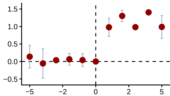
Figure 6: Coefficients relative to treatment time
