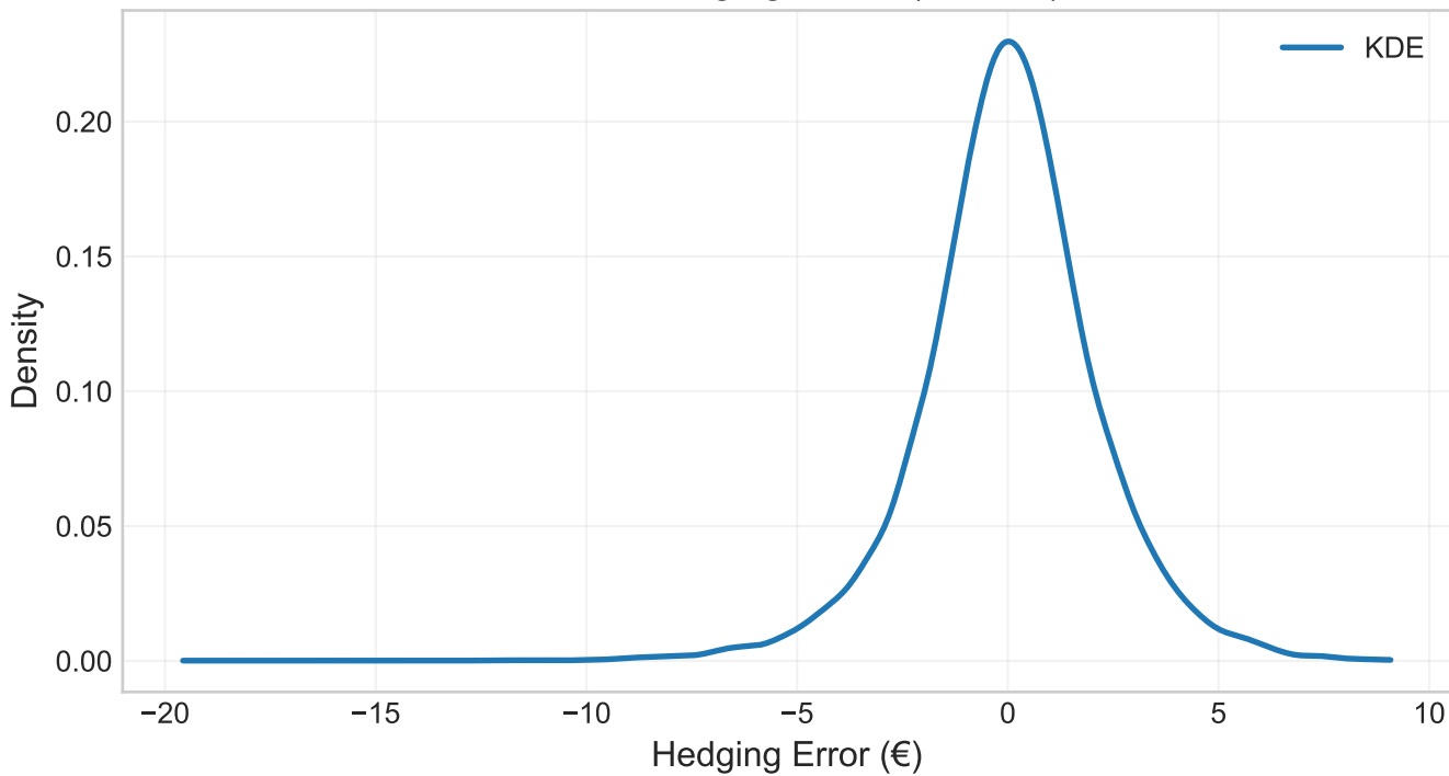
KDE of Hedging Errors (n=1000)
