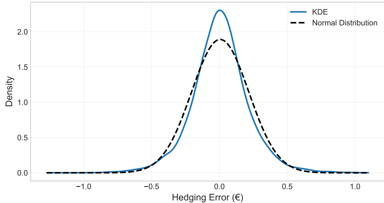
KDE vs Normal Distribution (n=100000)
