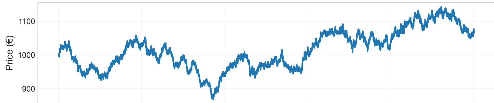
Underlying Price Process S_t (n = 100000 steps)
