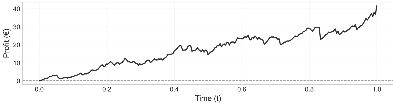
Cumulative P&L (n = 252 steps)
