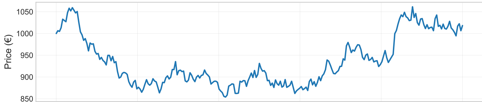
Underlying Price Process S_t (n = 252 steps)
