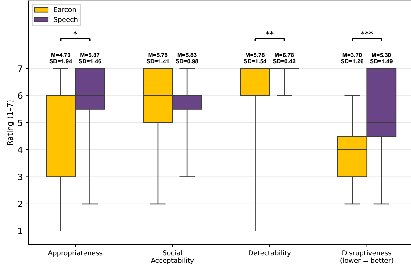
Math HIGH: Earcon vs Speech (chosen by AudioAdapt)
