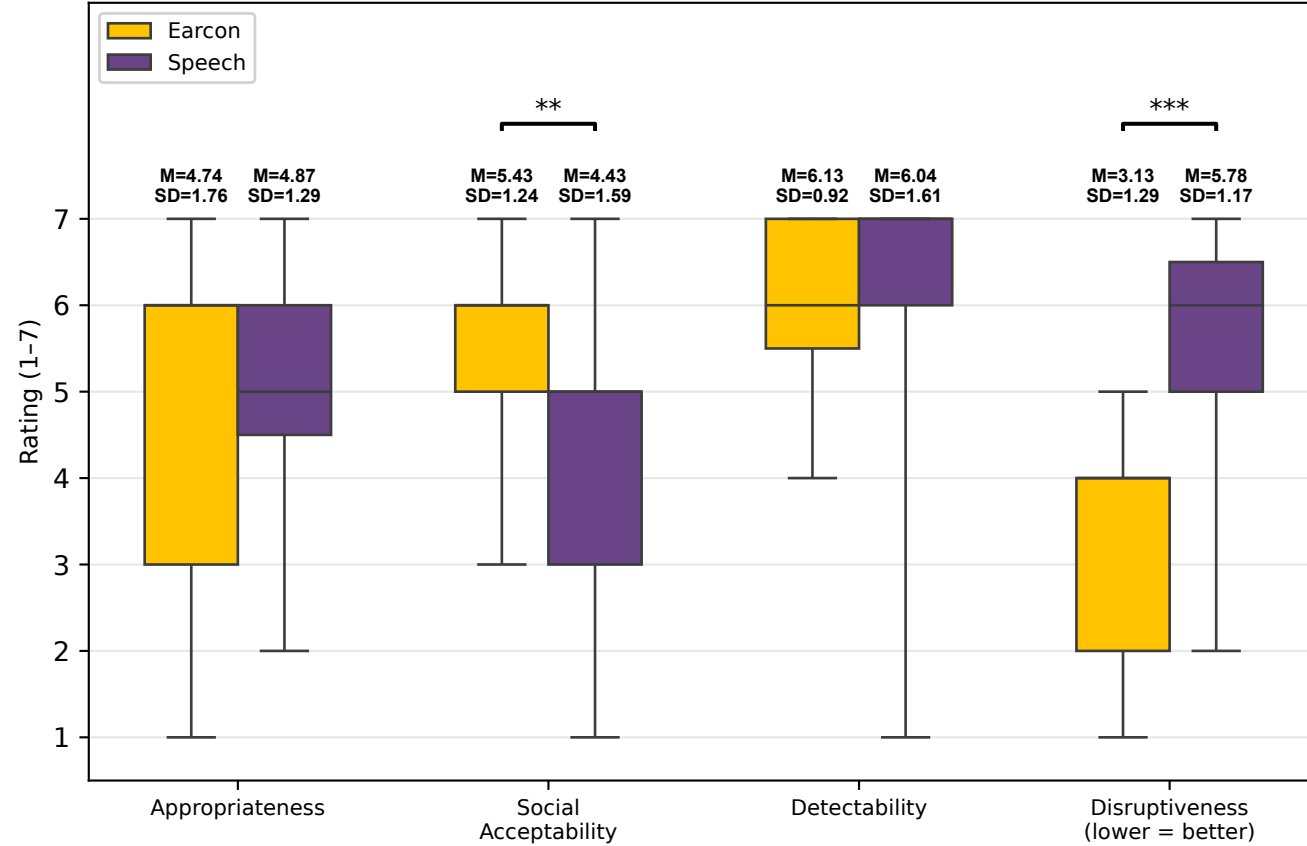
Interview HIGH: Earcon (chosen by AudioAdapt) vs Speech
