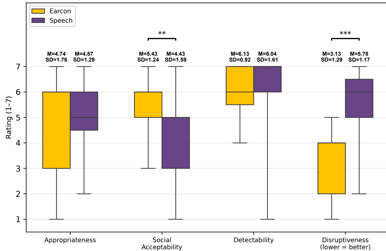
Interview HIGH: Earcon (chosen by SonoAdapt) vs Speech
