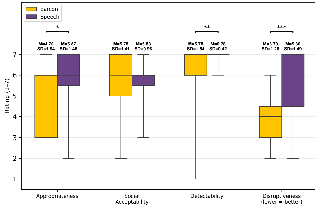
Math HIGH: Earcon vs Speech (chosen by SonoAdapt)
