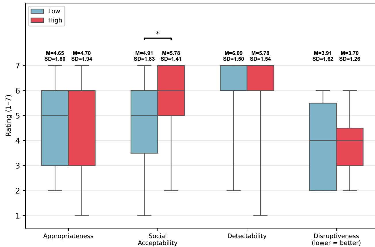
Math × Earcon
