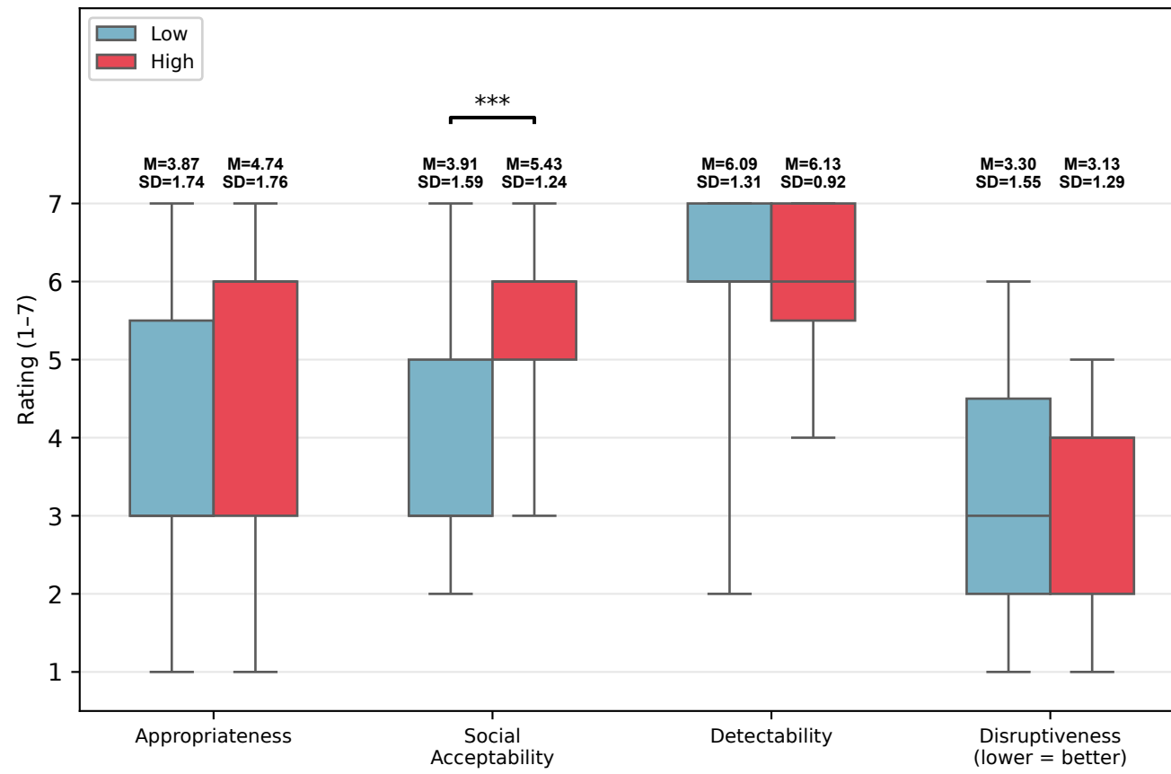
Math × Earcon
