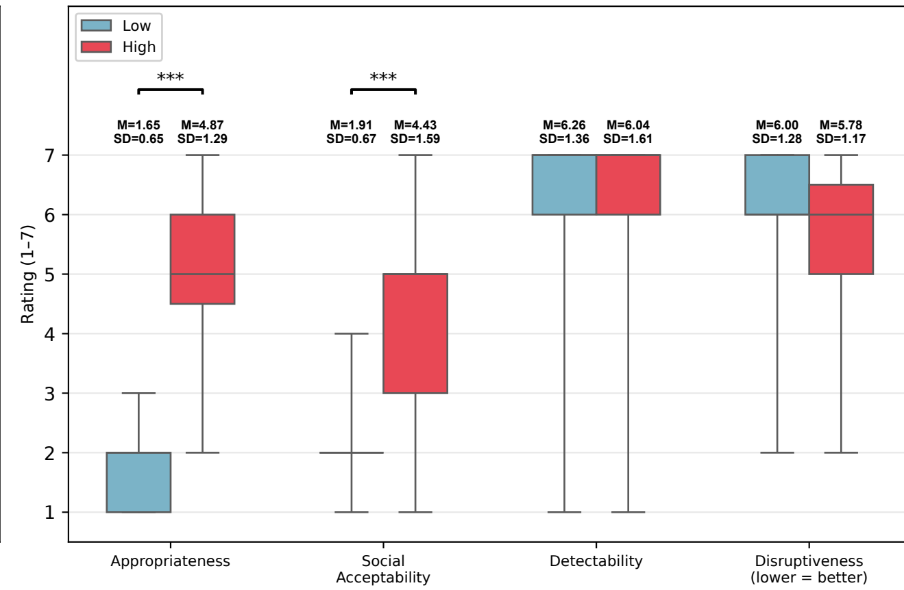
Math × Speech
