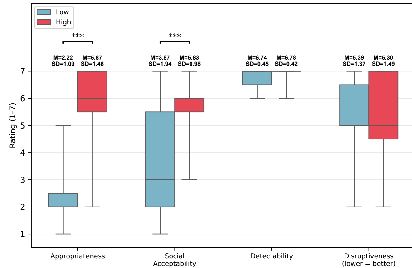
Math × Speech
