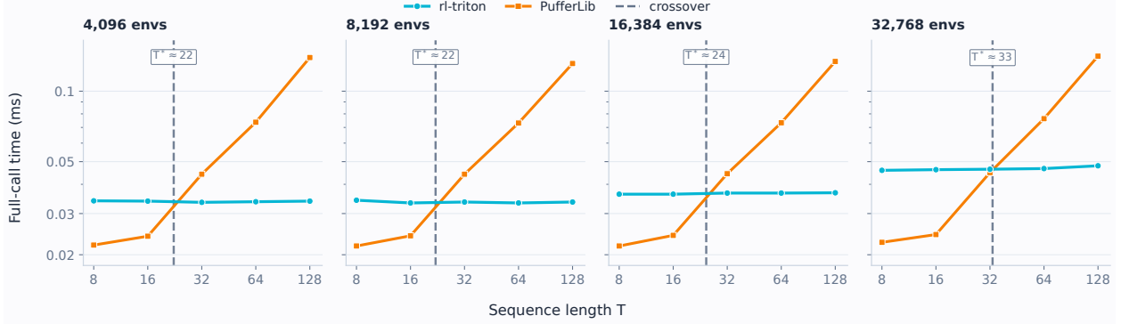
Figure 3: Full-call GAE performance of rl-triton and PufferLib in the massively parallel simulation regime on an H100. rl-triton has lower runtime at 11 of 20 shapes, including every configuration with seq_len \geq 32 except (\text{num\_envs}, \text{seq\_len}) = (32768, 32) ; PufferLib is faster at all configurations with seq_len \leq 16 . The crossover shifts to longer sequences as num_envs increases, reflecting PufferLib ’s low overhead for very short per-thread sequential scans.
