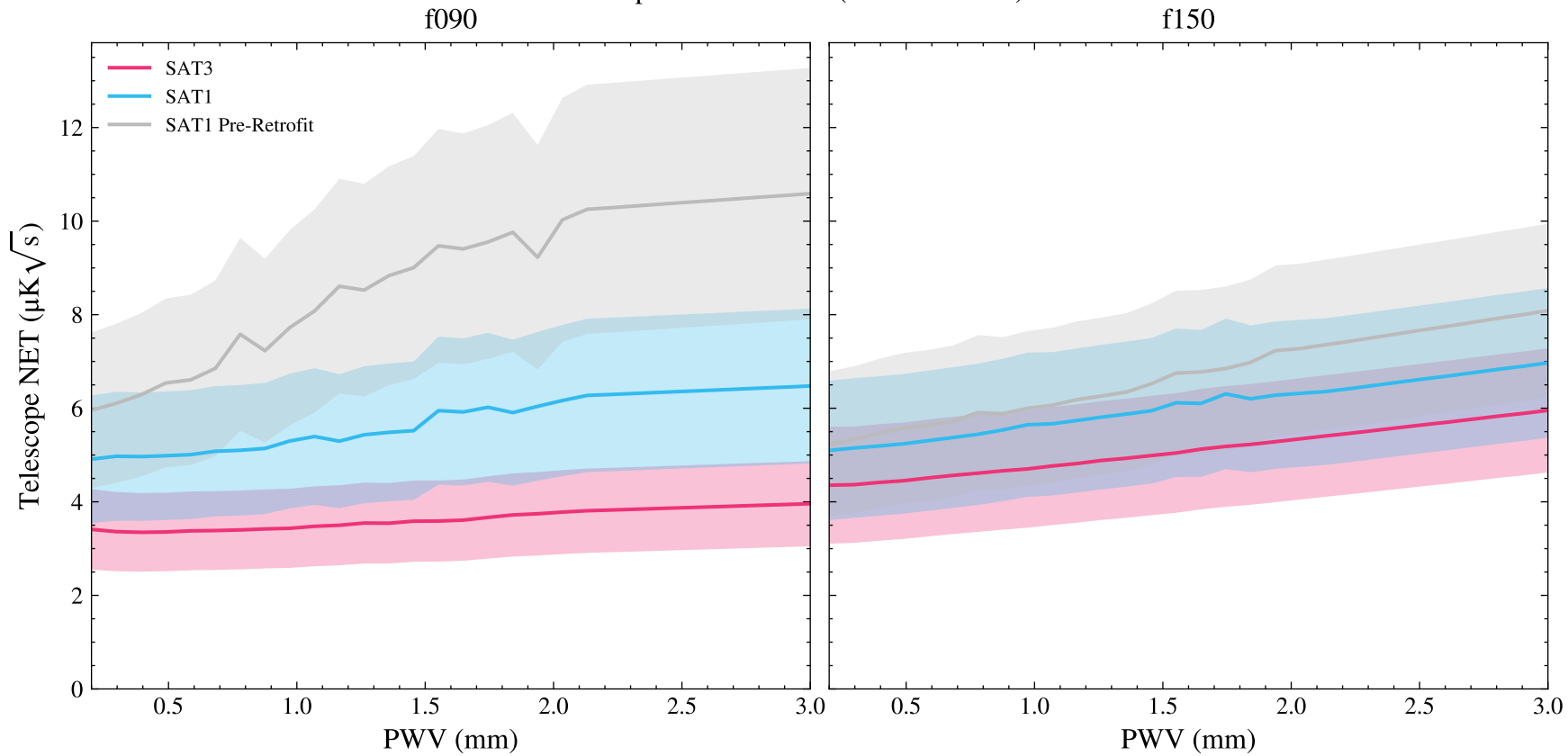
Telescope NET vs PWV (elevation=60°)
