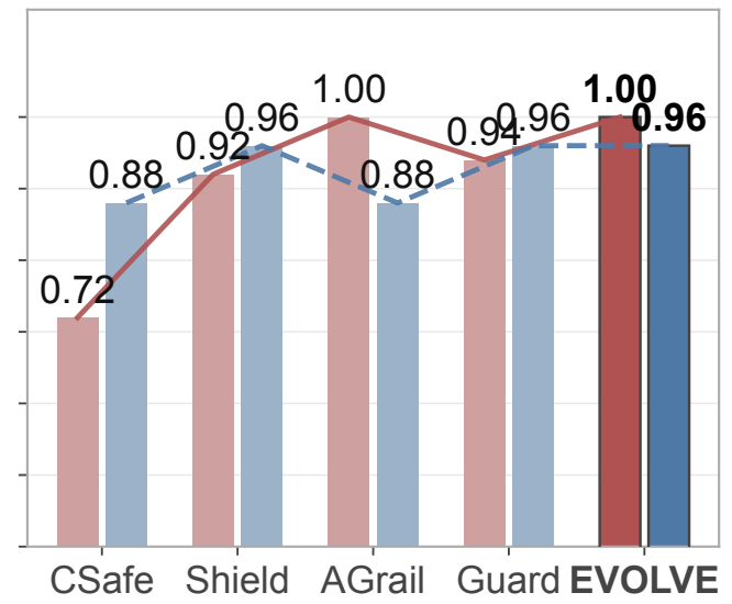
Jailbroken
