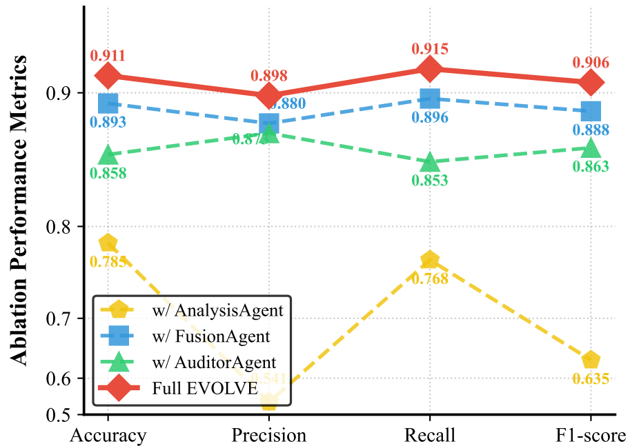
(b) Ablation Study
