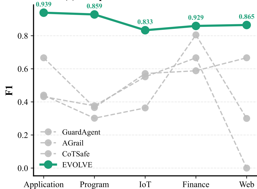
(a) Comparison on Different Domains
