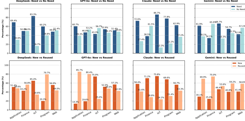
Fig. 3: Results for EVOLVE’s evolving process on R-Judge benchmark. EVOLVE can dynamically determine which tasks need security tools. Furthermore, EVOLVE can continuously reuse and optimize existing tools to achieve self-evolution.
