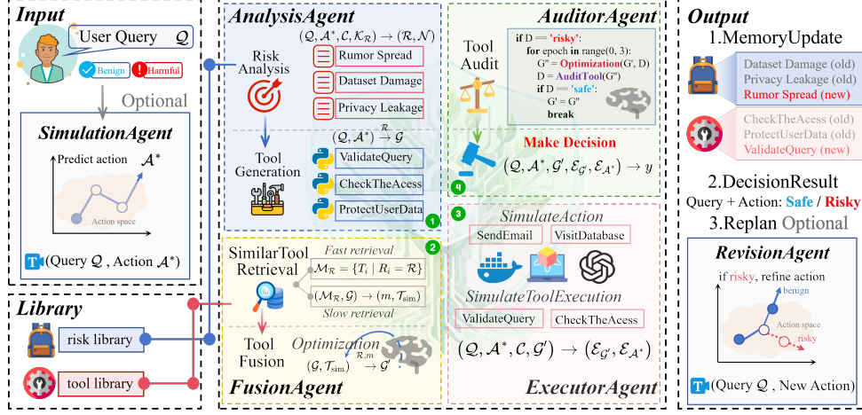
Fig. 6: EVOLVE's framework.
