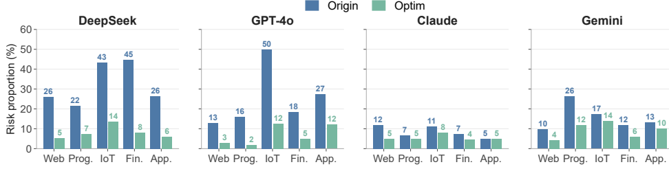
Fig. 4: Results for EVOLVE’s auditing mechanism on R-Judge benchmark. Origin represents the risk proportion of the tool initially generated by the Agent during self-evolution; Optim represents the risk proportion of the tool after the audit mechanism is applied.
