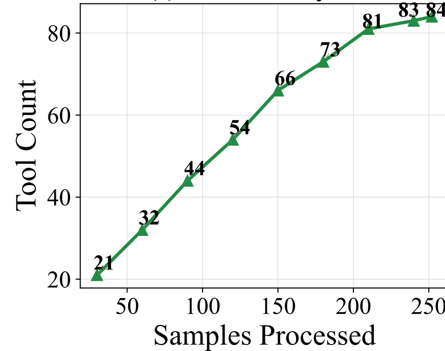
(c) Tool Library Size
