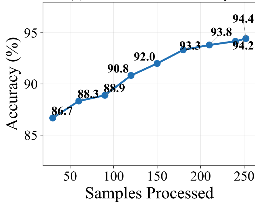
(a) Cumulative Accuracy
