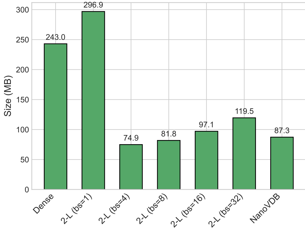
Memory Footprint
