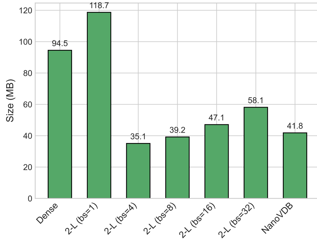
Memory Footprint
