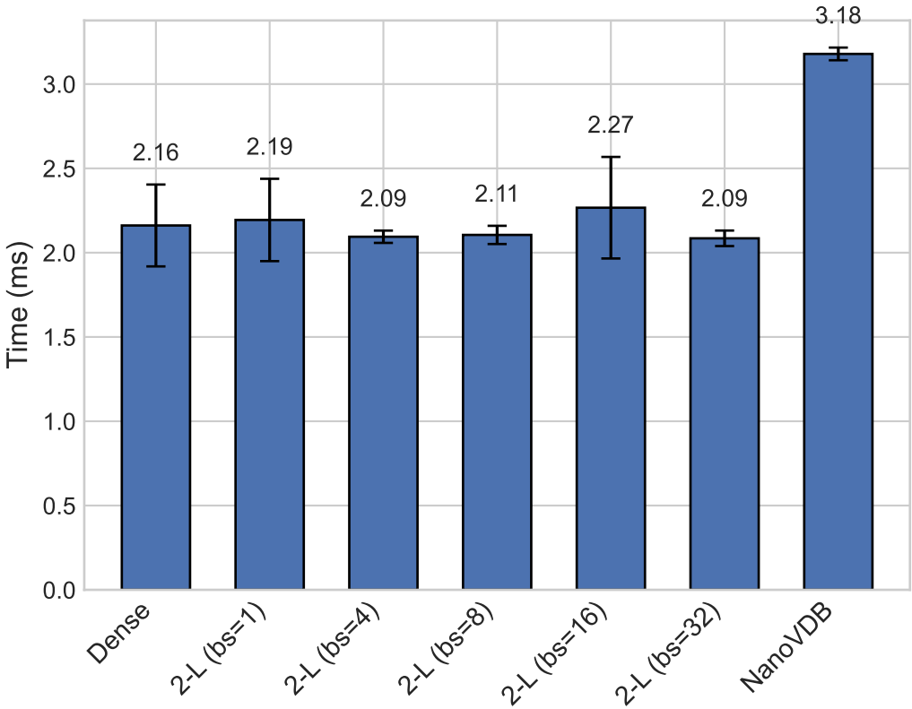
Query Time per Batch (mean \pm std)
