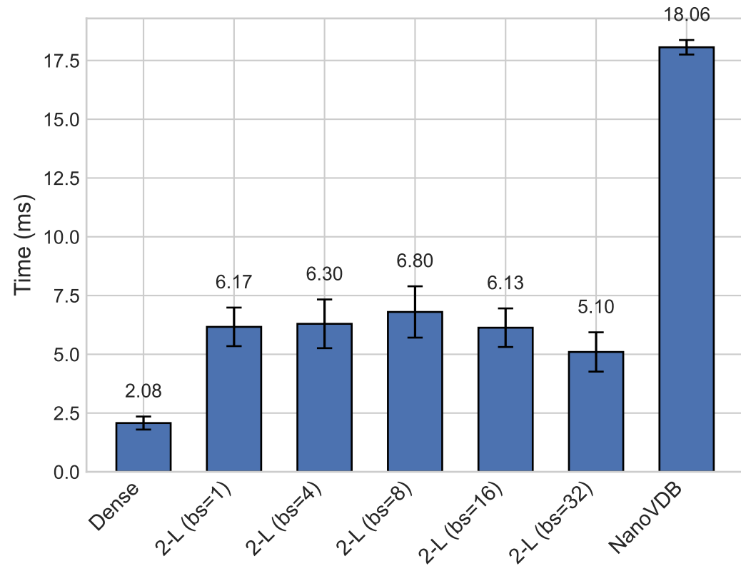
Render Time per Frame (mean \pm std)
