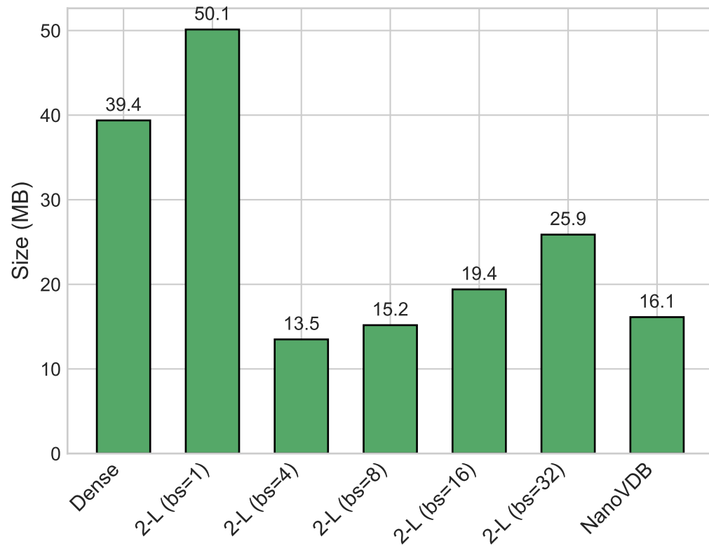
Memory Footprint
