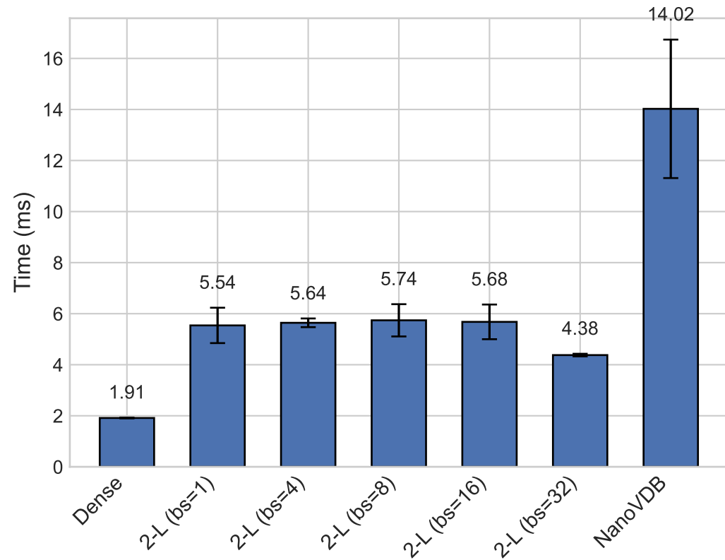
Render Time per Frame (mean \pm std)
