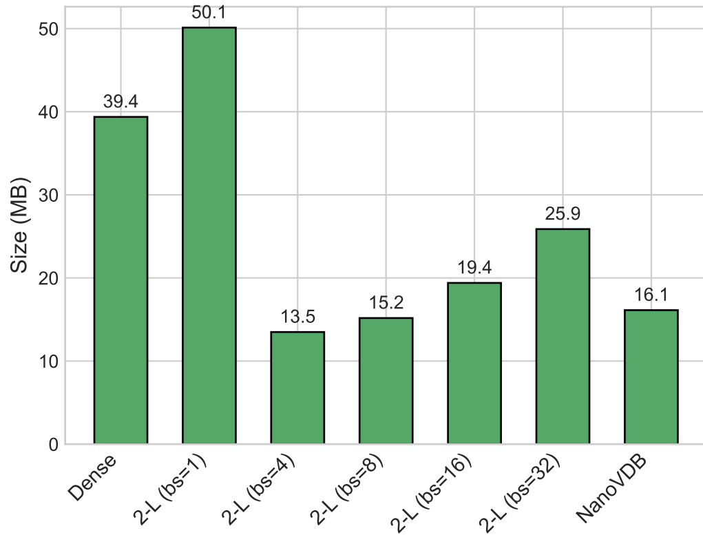
Memory Footprint
