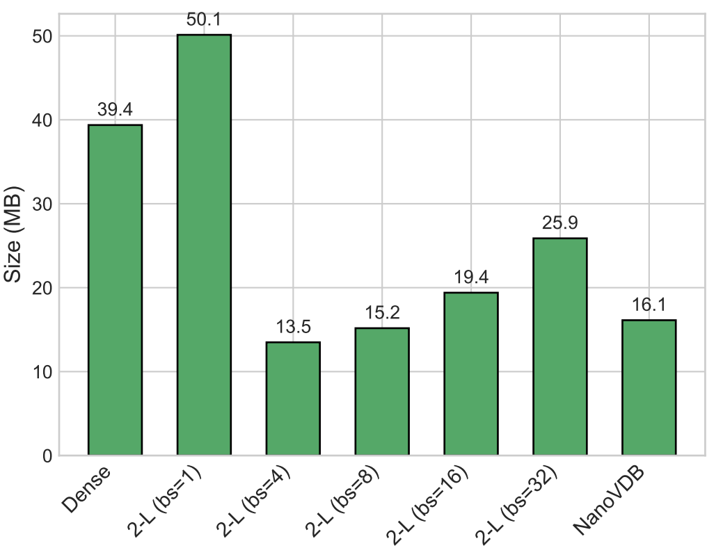
Memory Footprint
