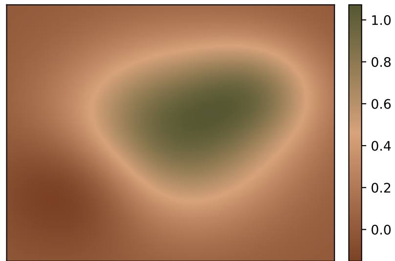
heatmap (palette as colormap)
