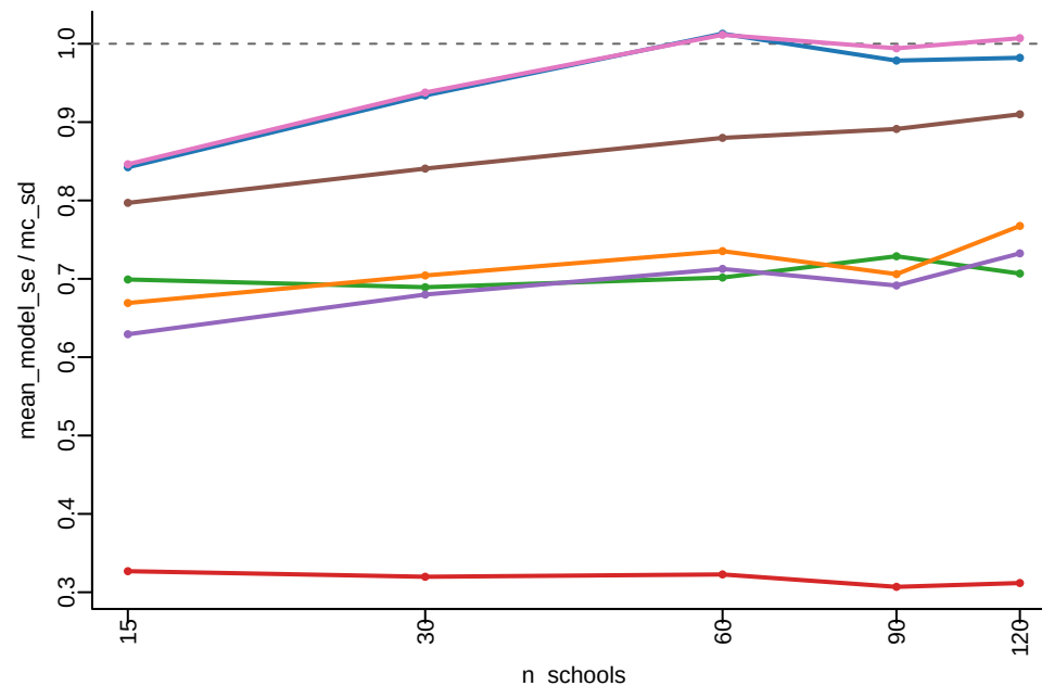
Model A : Fixed-Effect SE Calibration
