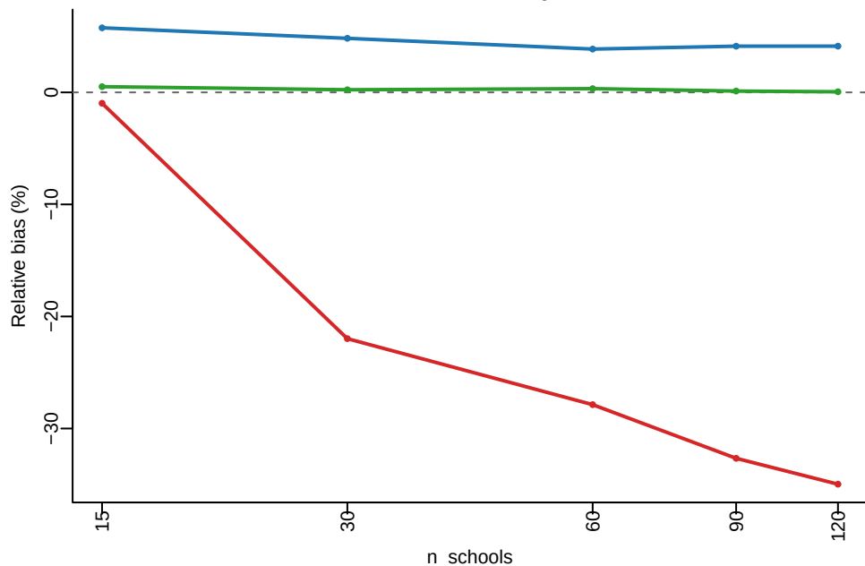
Model A : Variance-Component Bias
