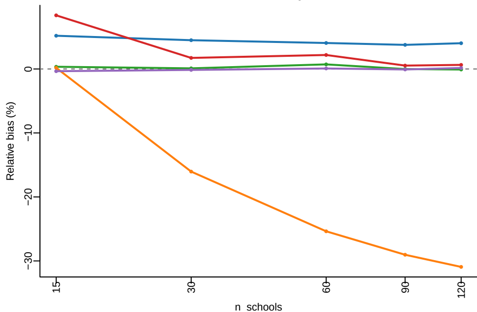
Model B : Variance-Component Bias
