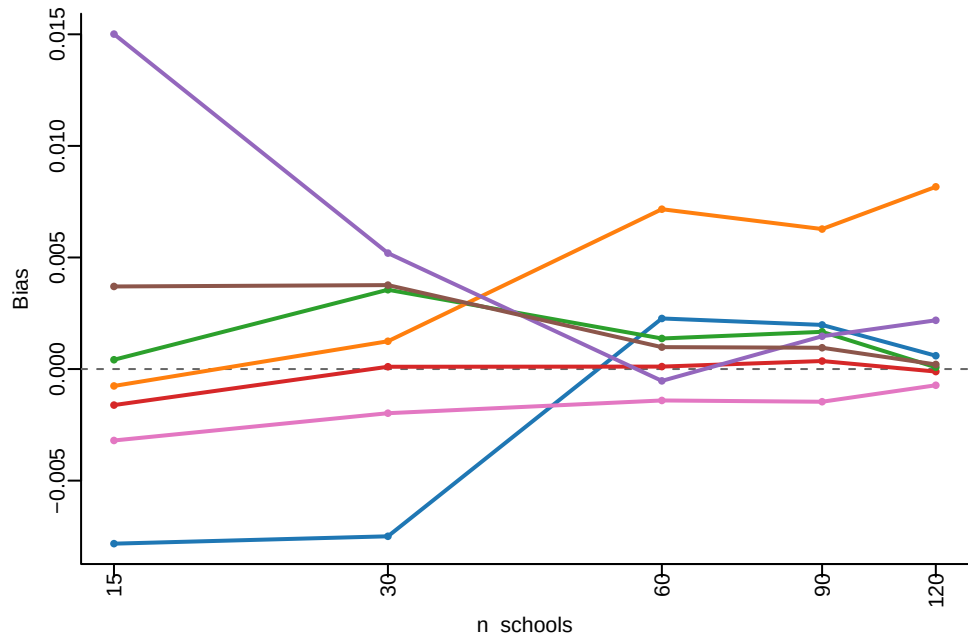
Model B : Variance-Component Bias
